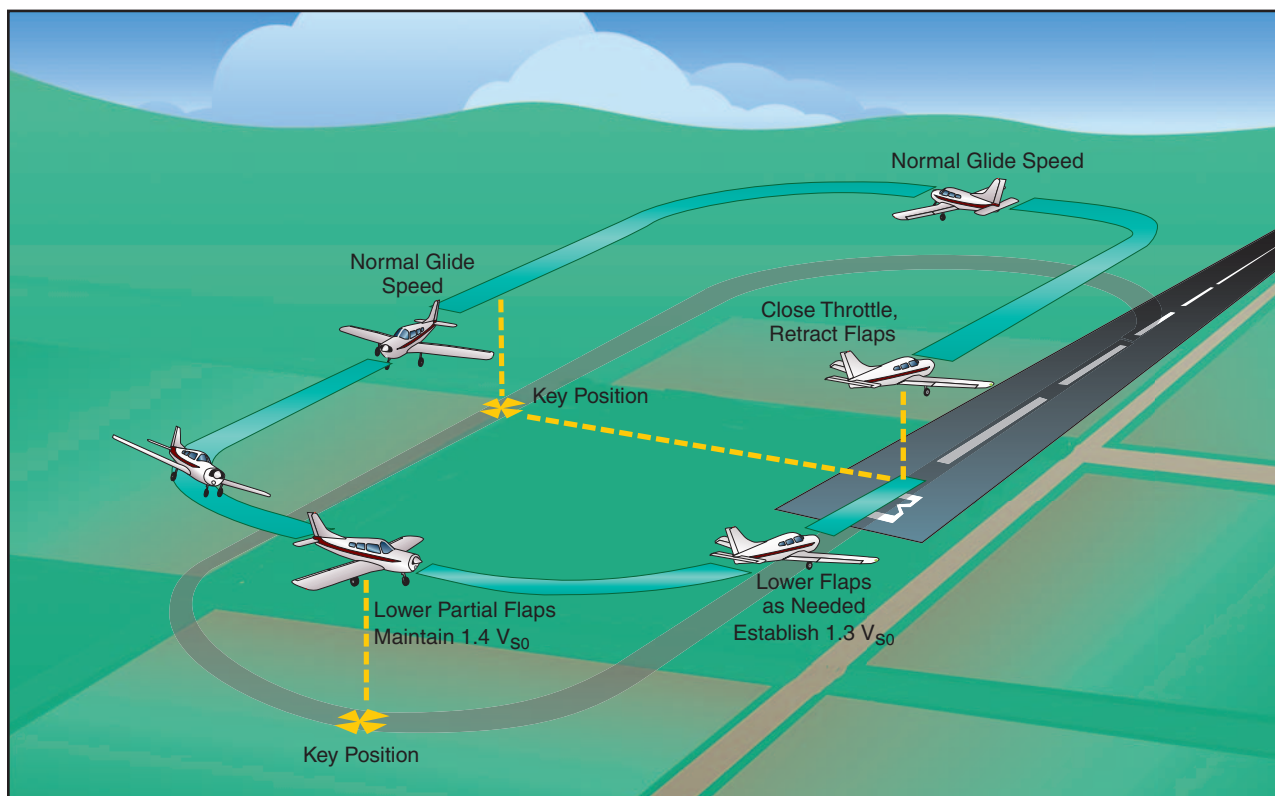
Figure 8-28. 360° power-off approach.
