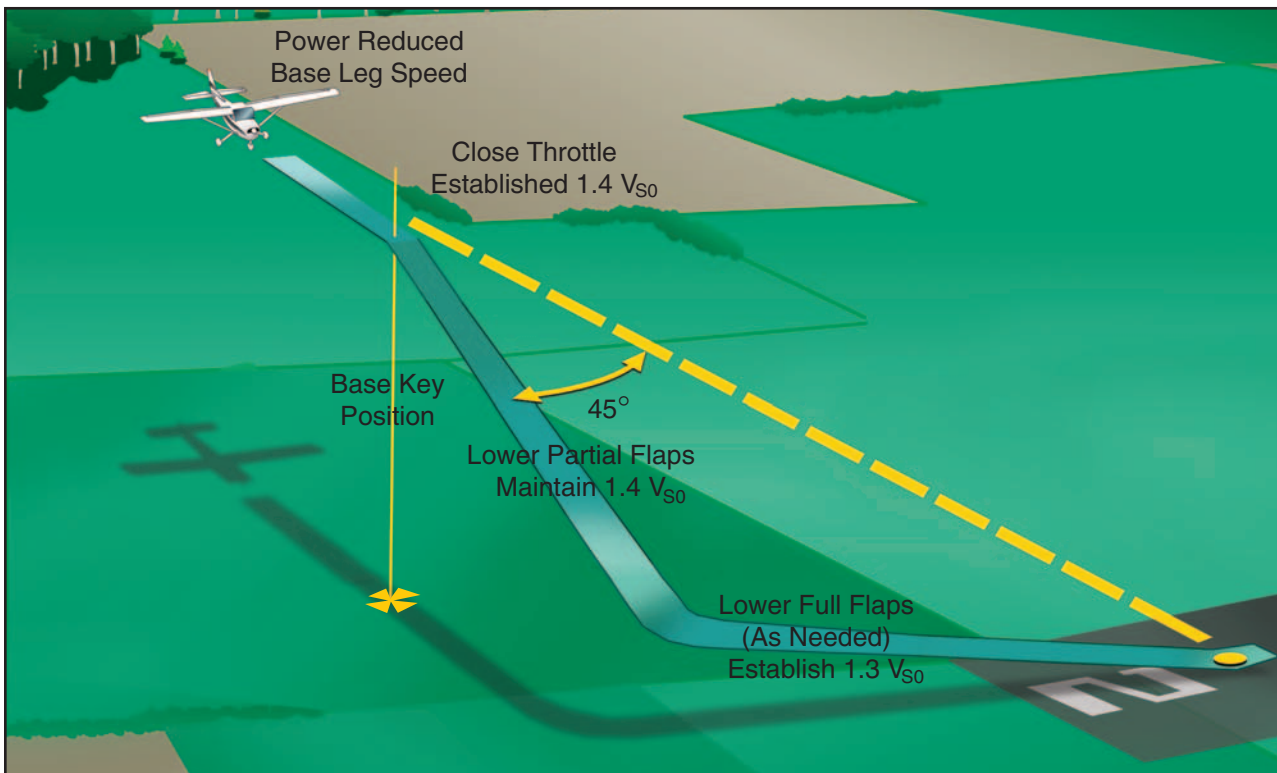
Figure 8-26. 90° power-off approach.
