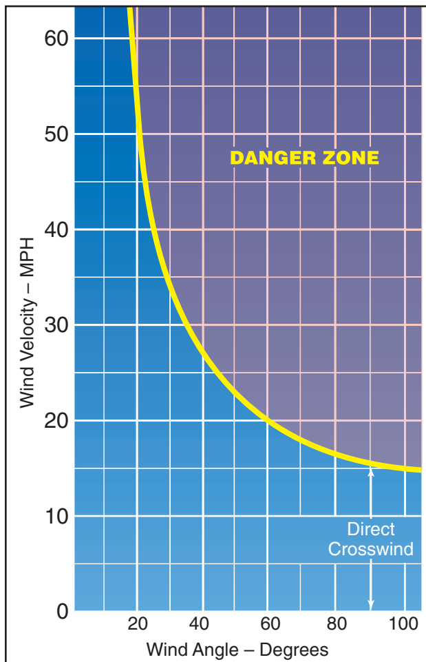
Figure 8-18. Crosswind chart.
