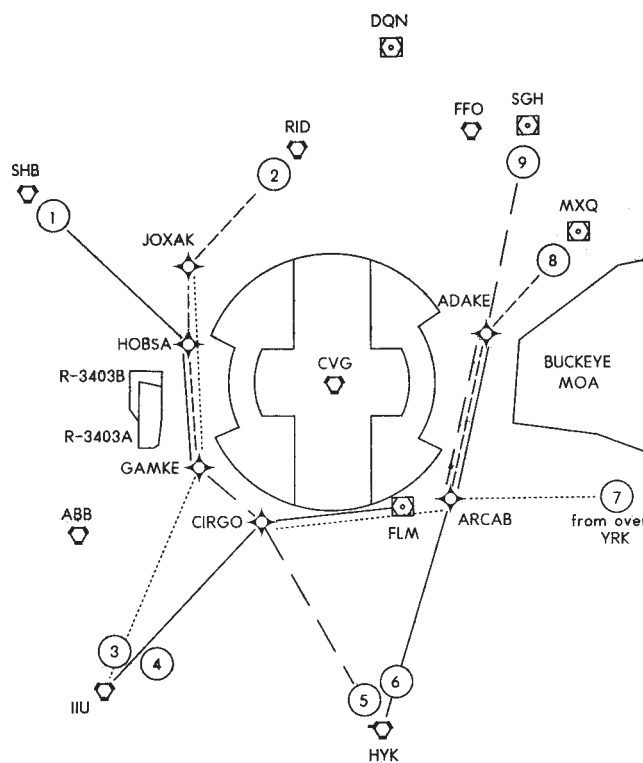
Figure 10. RNAV IFR Terminal Transition Routes
