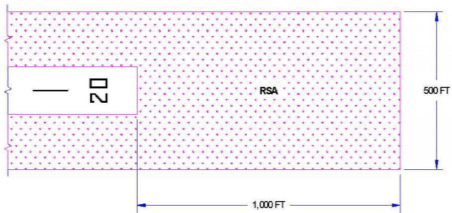
STANDARD (APPROACH CATEGORY C &amp; D)
